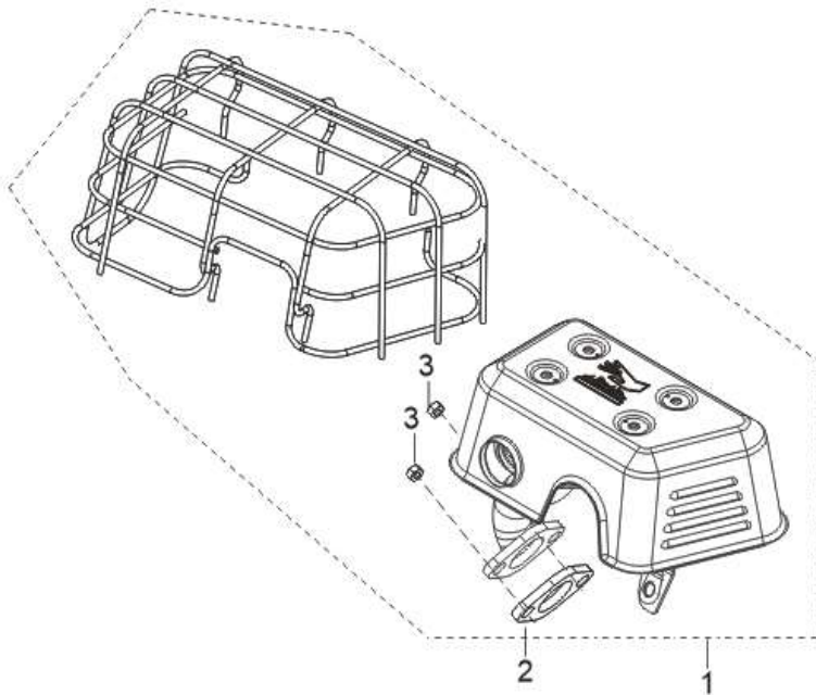
FIG.13 MUFFLER ASSY. (F02)
