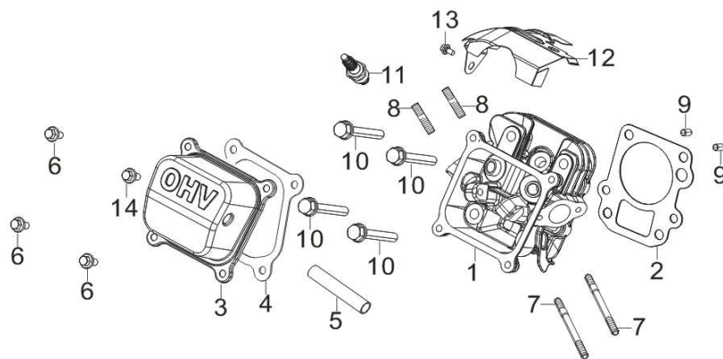
FIG.3 HEAD SUBASSEMBLY, CYLINDER / PLUG, SPARK (E03)
