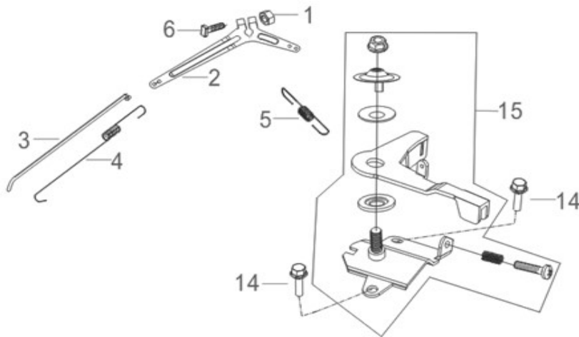
FIG.11 CONTROL ASSY, THROTTLE (E11)
