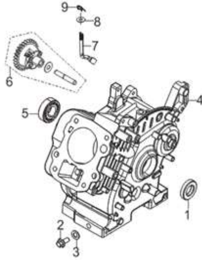
FIG.1 CRANKCASE. / GEAR ASSY, GOVERNOR. (E01)
