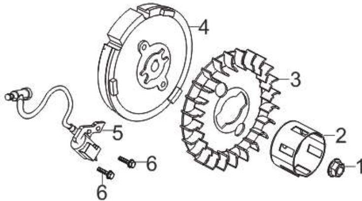
FIG.10 FLYWHEEL / IMPELLER / STARTER PULLEY / IGNITION COIL (E10)
